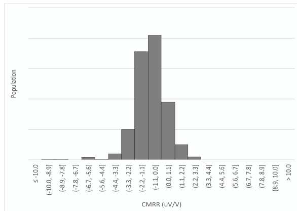
Figure 5d. Common Mode Rejection Ratio Distribution, G200
