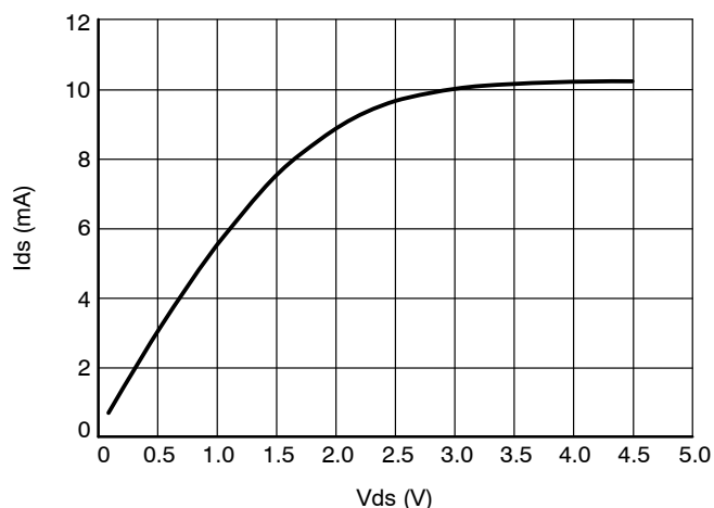
Figure 21. Power Good Current vs. Drain-to-Source Voltage
