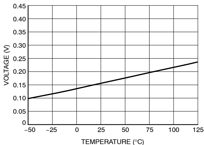
Figure 19. Power Good Saturation Voltage vs. Temperature
