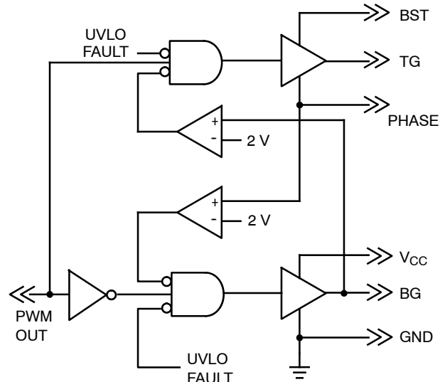
Figure 24. Block Diagram
