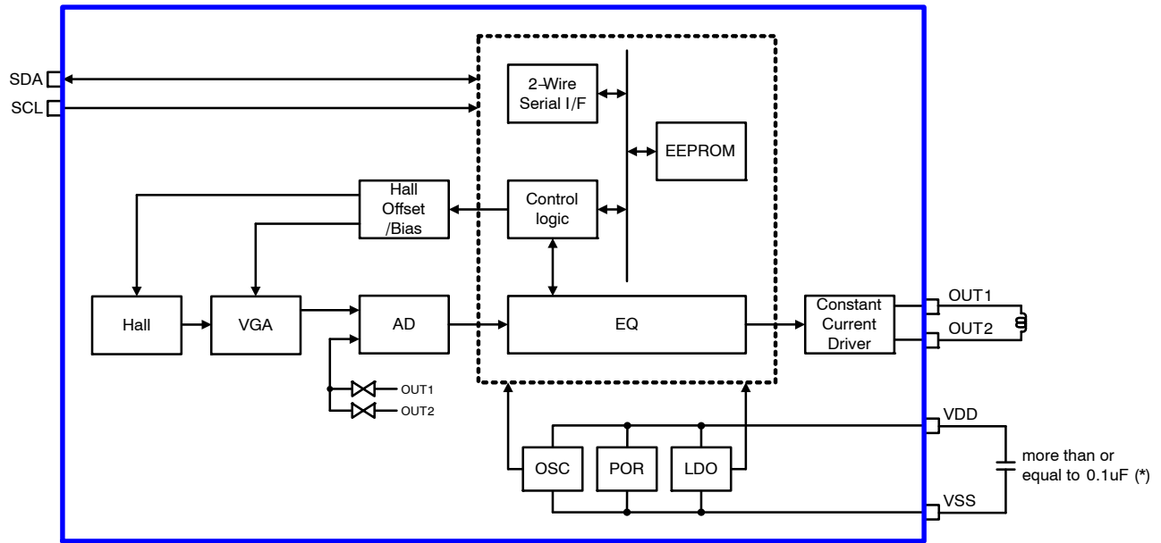
Figure 1. Block Diagram
