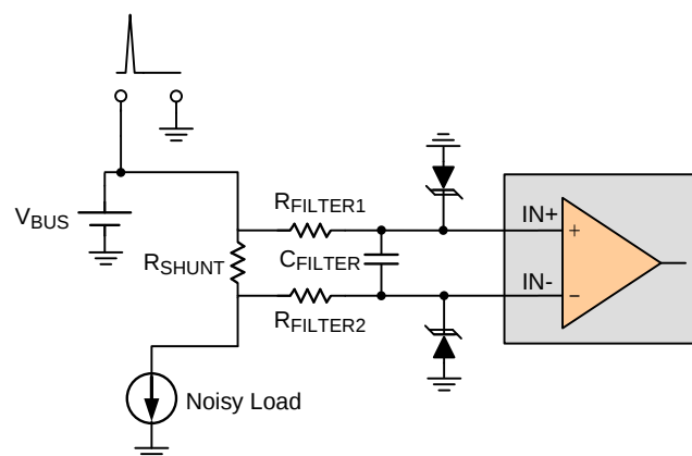
Figure 8. RTQ6056 with Input Protection
